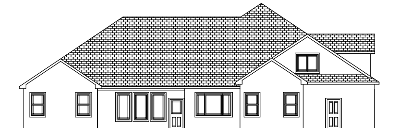
Back Elevation
